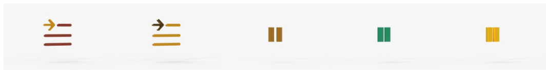
Paragraph_B
