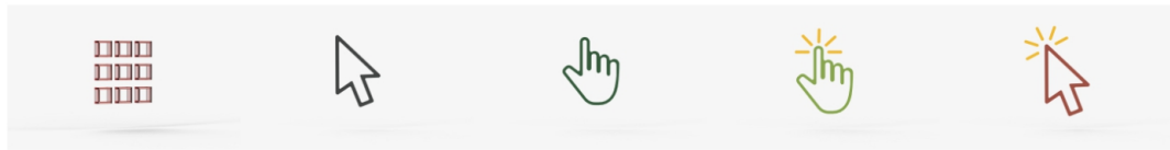
Icon_C_8
