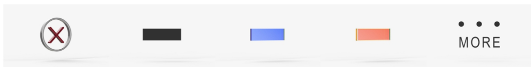
Message_Error_C
