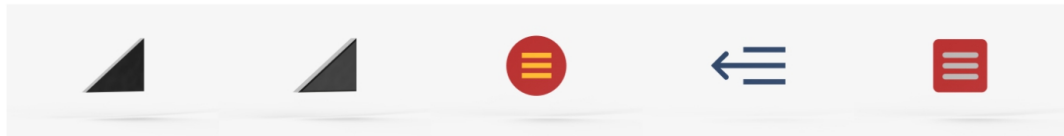
Full_Signal_Streight_B_1_01
