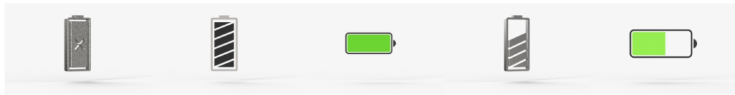
Battery_Low_C_4
