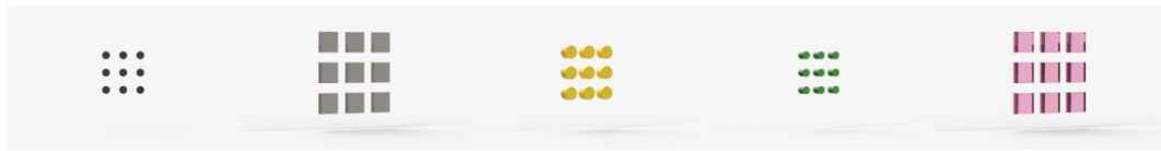
Apps_A_2_1
