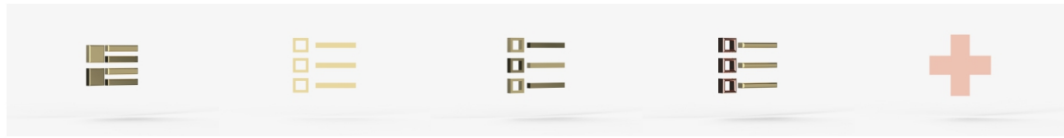
Multi_Select_C
