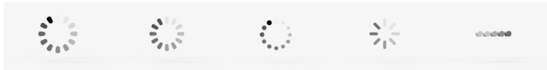
Status_Bar_A_3
