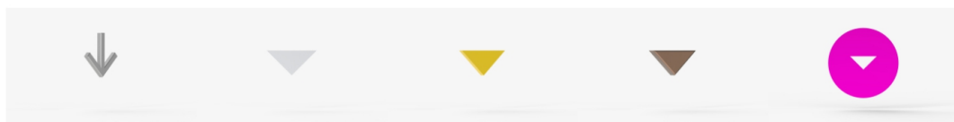
Arrow_Downward_C
