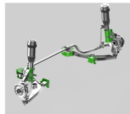
Front_Suspension
