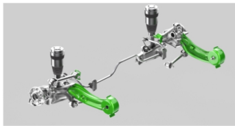
Rear_Suspension
